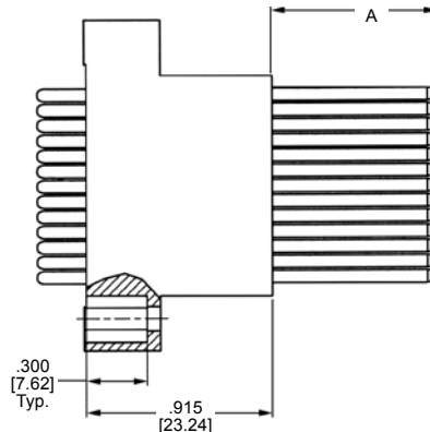
Plug Assembly
