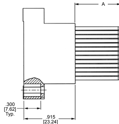
Receptacle Assembly
