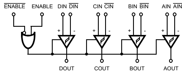
Figure 3. Logic Diagram
