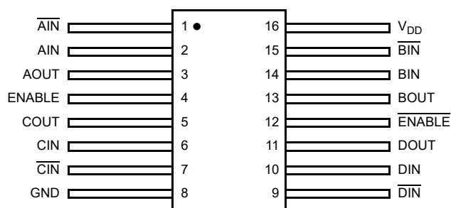
Figure 2. 16 LD FLATPACK, MIL-STD-1835: CDFP4-F16 Top View [1][2][3]
