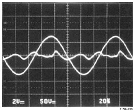
Figure 15. 0.3% THD at 10kHz, P_O = 350W , R_L = 8\Omega
