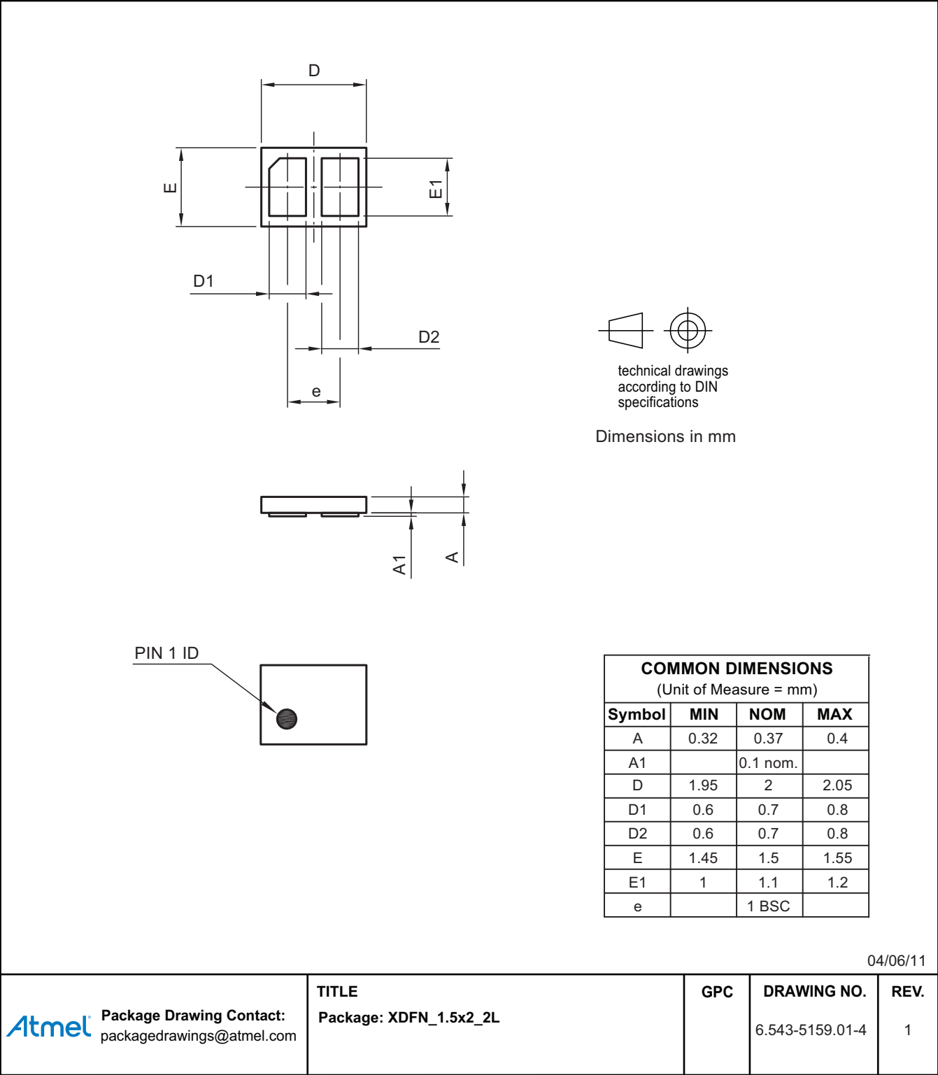
Figure 11-7. XDFN Package
