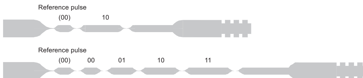
Figure 5-15. 1-of-4-coding Protocol
