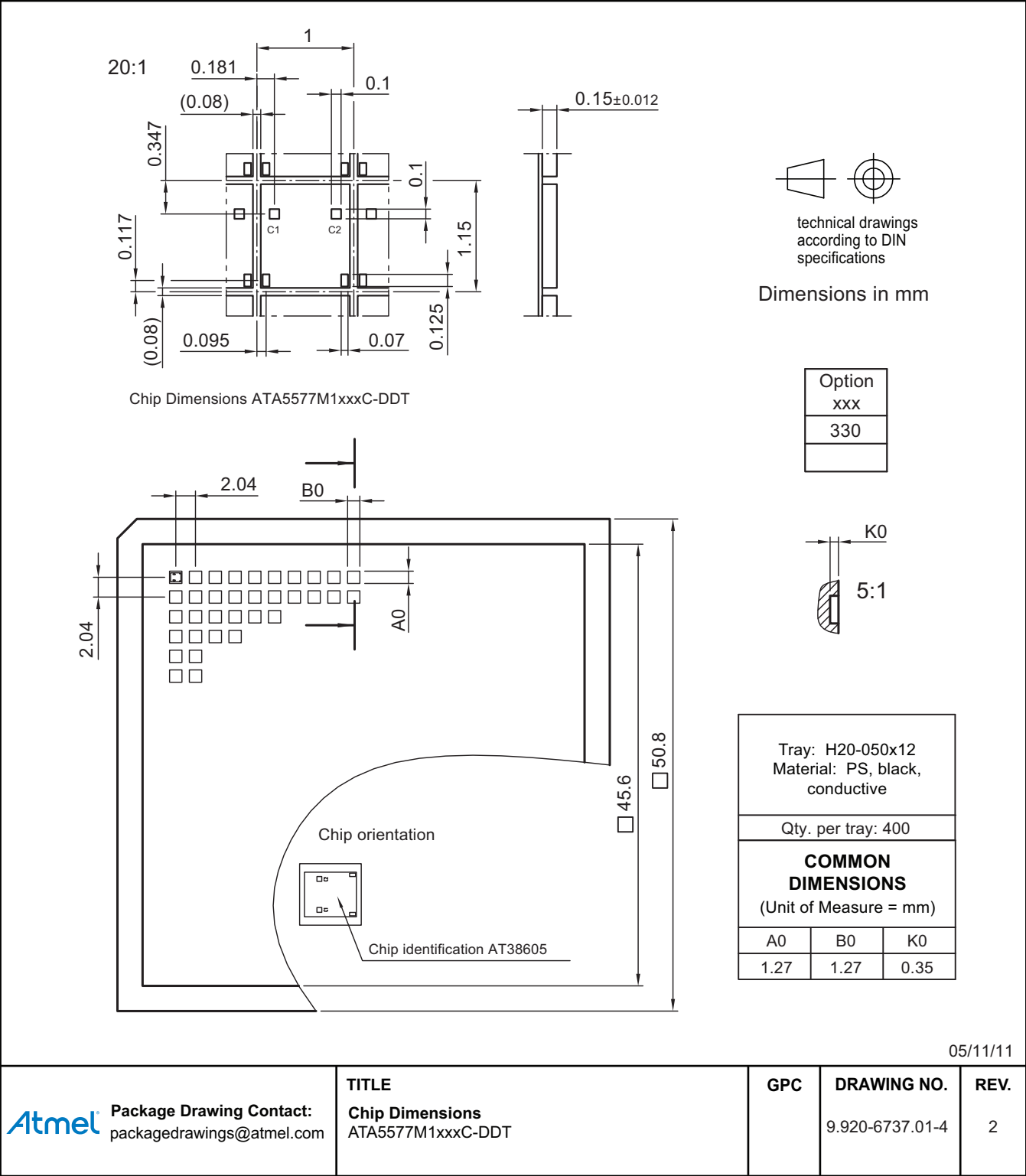
Figure 11-2. Die in Waffle Pack
