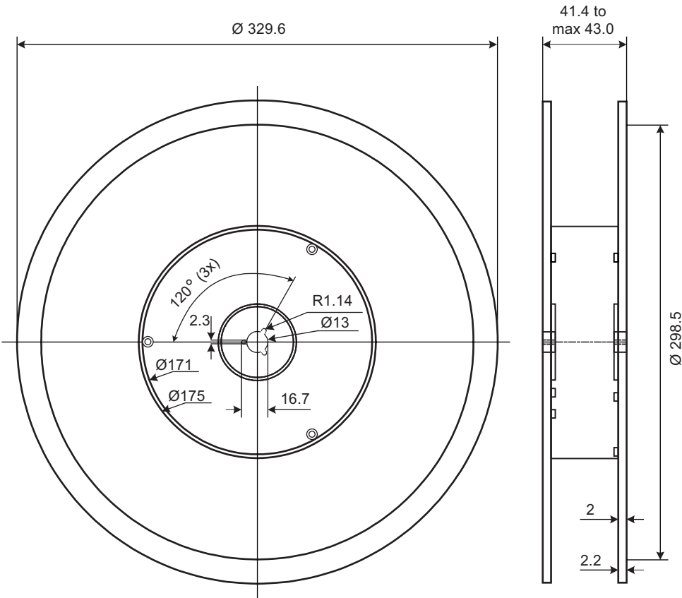
Figure 11-6. Shipping Reel for NOA3 Micromodule
