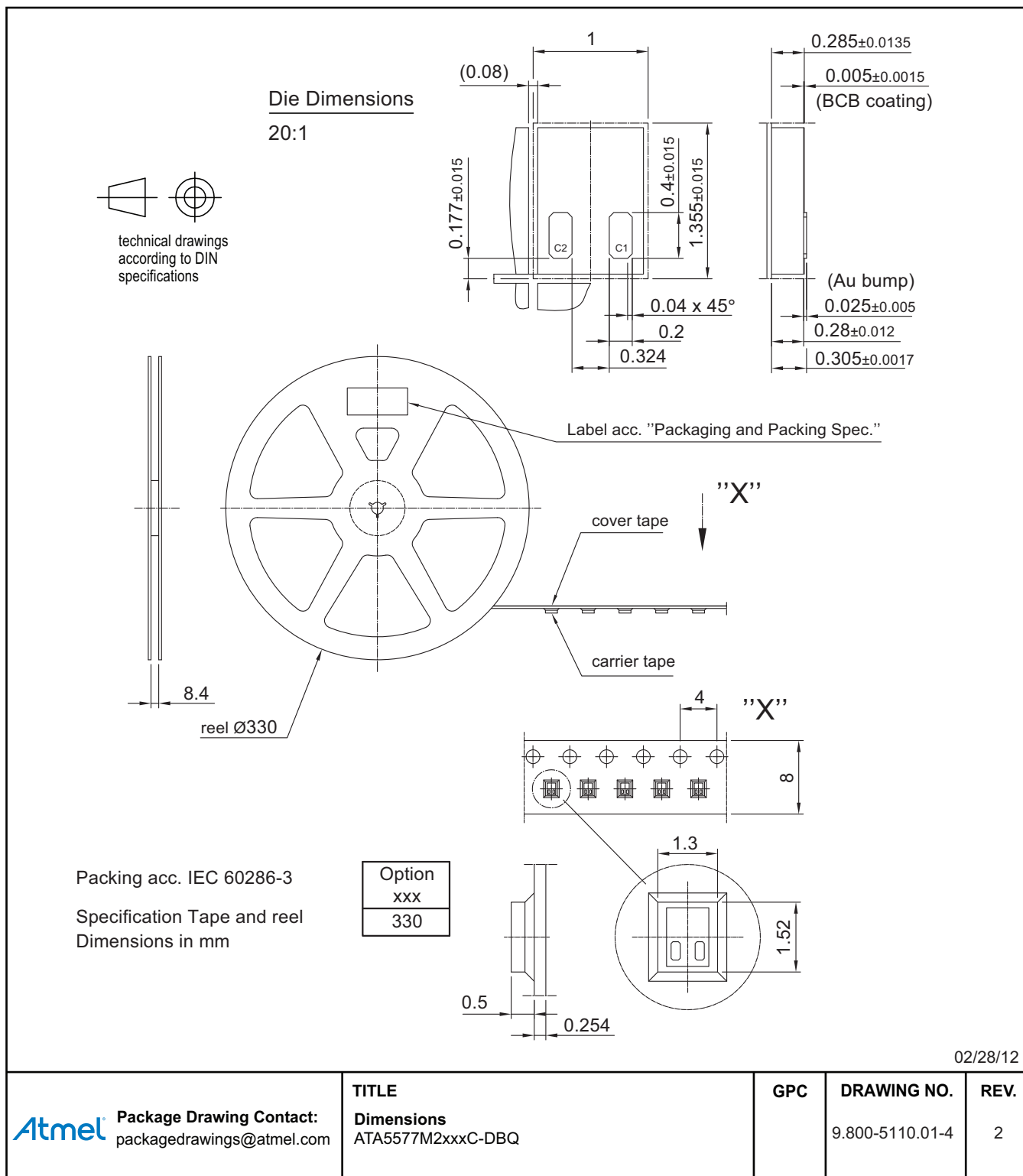
Figure 11-4. Die in Blister Tape
