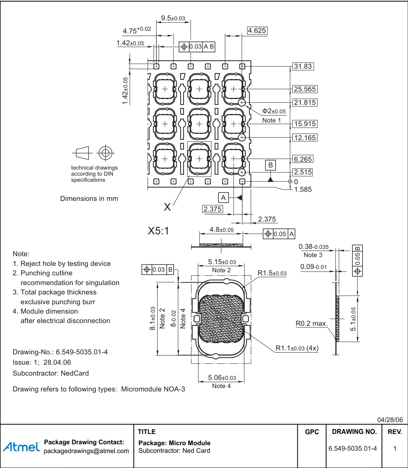
Figure 11-5. NOA3 Micromodule
