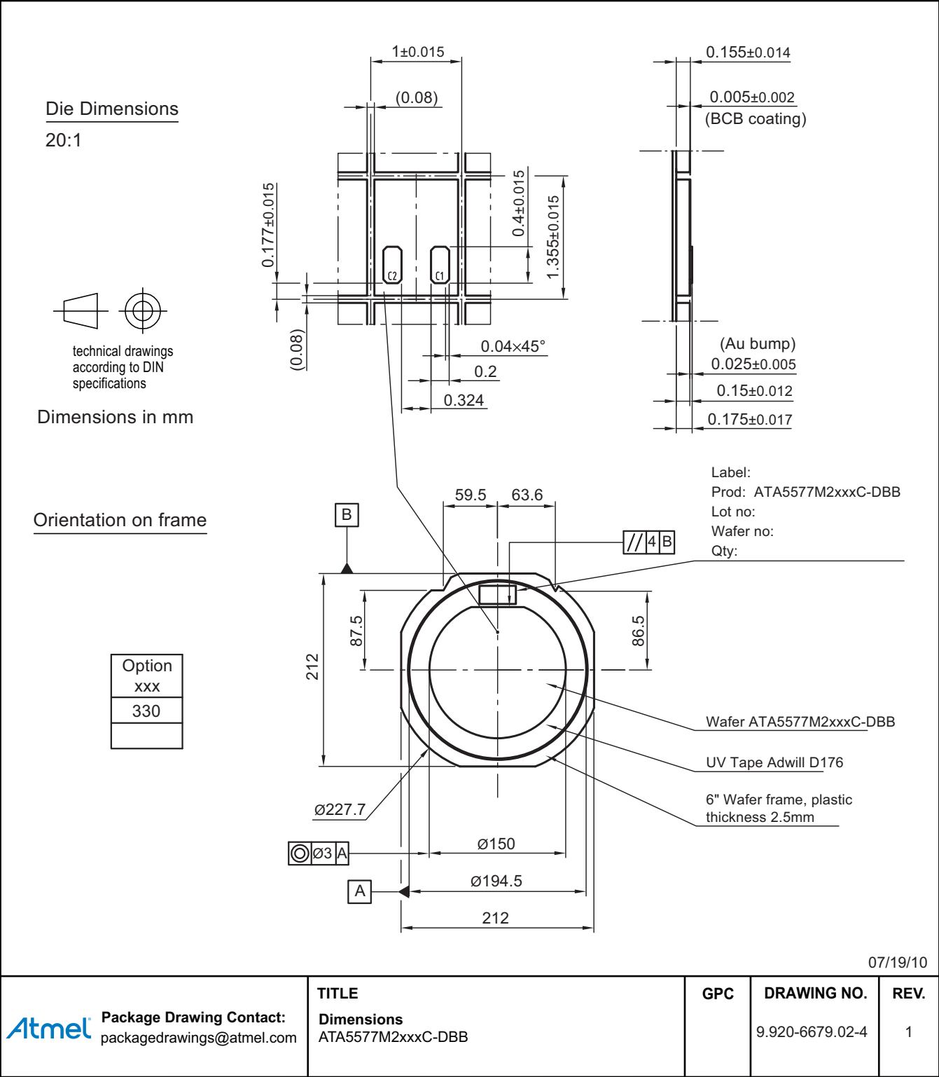
Figure 11-3. Sawn Wafer on Foil with Ring (Type 2, Mega Pads and Au Bumps)
