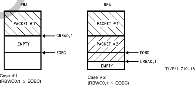
FIGURE 5-4. Receive Resource Area Format
