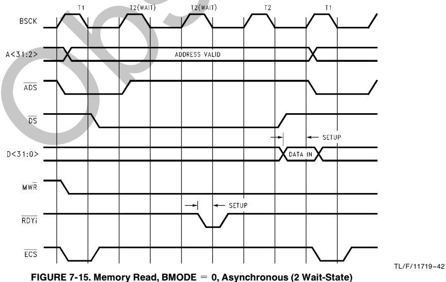
FIGURE 7-15. Memory Read, BMODE = 0, Asynchronous (2 Wait-State)
