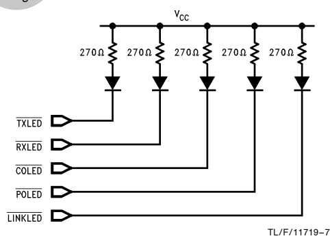
FIGURE 3-4. Typical SONIC-T LED Connection
