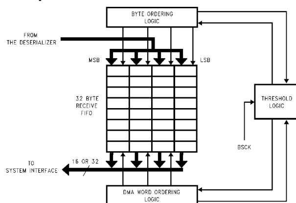
FIGURE 3-8. Receive FIFO
