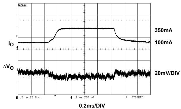
FIGURE 8. TRANSIENT RESPONSE
