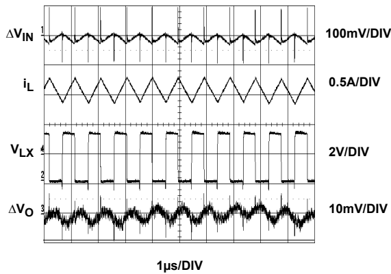
FIGURE 9. STEADY-STATE
