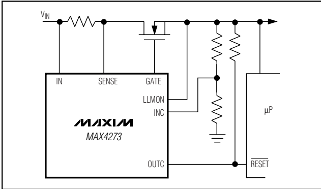
Figure 12. Power-On Reset
