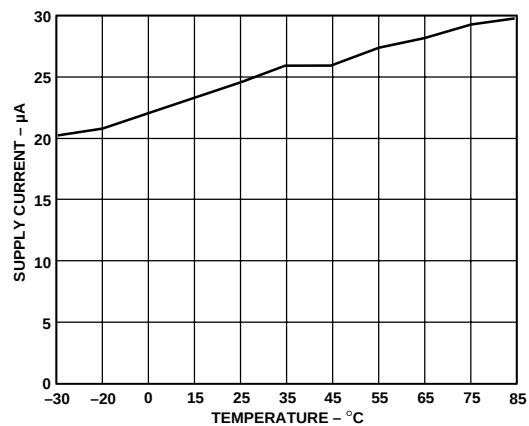
Figure 21. Supply Current vs. Temperature
