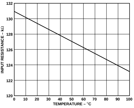
Figure 18. SU2 Input Resistance vs. Temperature
