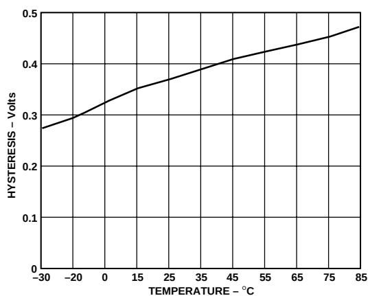
Figure 2. Hysteresis vs. Temperature for SU1—High to Low
