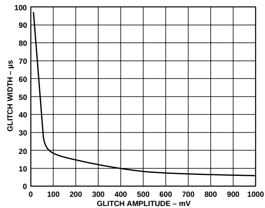
Figure 22. Glitch Immunity
