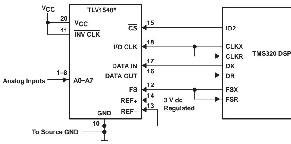
Figure 38. Typical Interface to a Microprocessor
