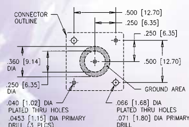
PCB LAYOUT (COMPONENT SIDE OF BOARD)
