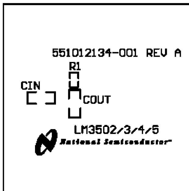
Figure 7. Bottom Silk Screen
