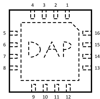
Figure 5. 16-Thin WQFN (RGH0016A)
