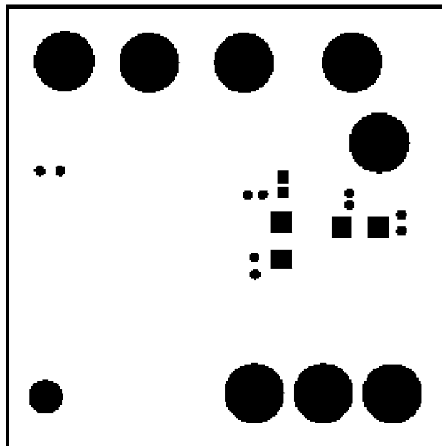
Figure 11. Bottom Pads
