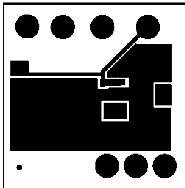
Figure 9. Bottom Traces
