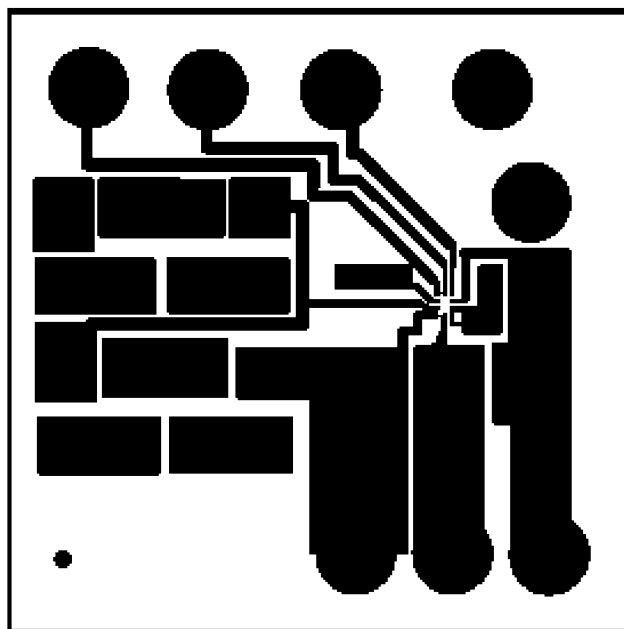
Figure 8. Top Traces
