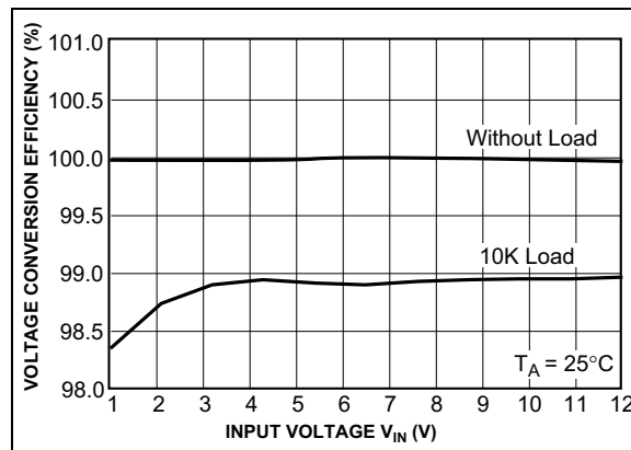
FIGURE 2-5: Voltage Conversion.
