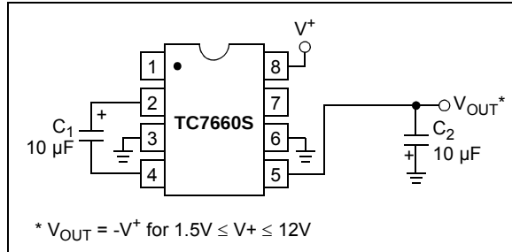
FIGURE 5-1: Simple Negative Converter.
