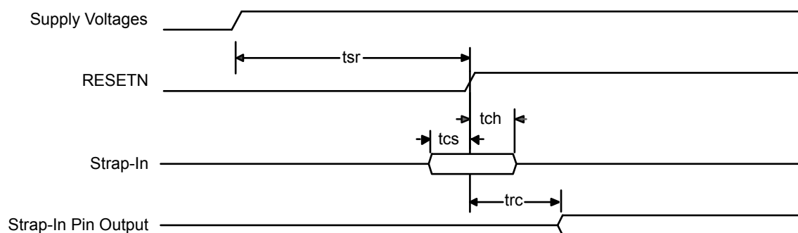
Figure 11. Reset Timing
