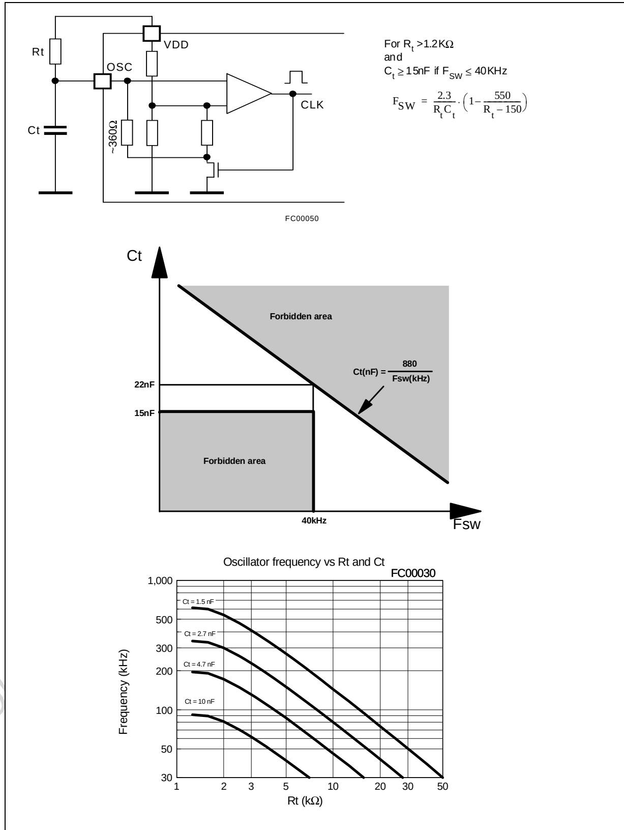
Figure 12. Oscillator
