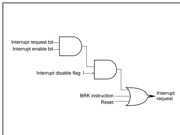
Fig. 8.3.1 Interrupt Control
