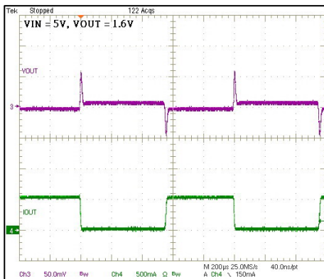
Figure 05. Load Transient
