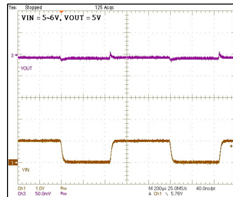
Figure 06. Line Transient
