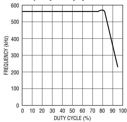
Frequency vs Duty Cycle
