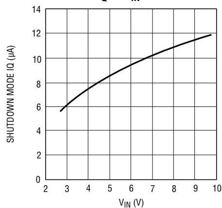
Shutdown I_Q vs V_{IN}
