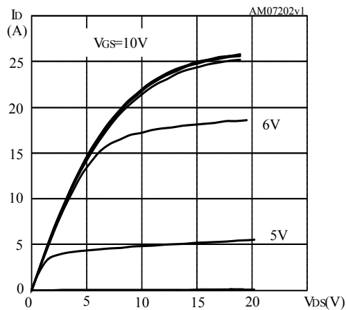
Figure 3. Output characteristics
