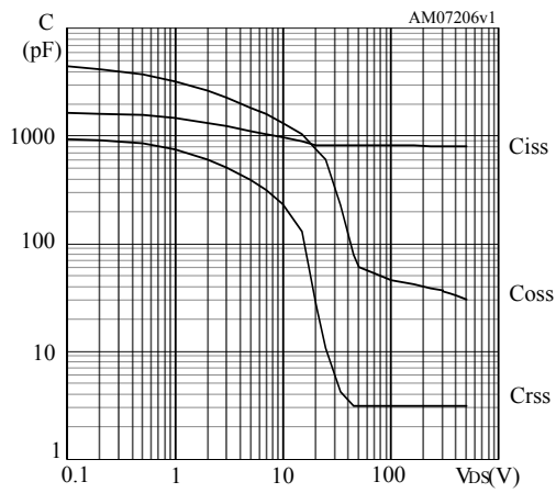
Figure 7. Capacitance variations
