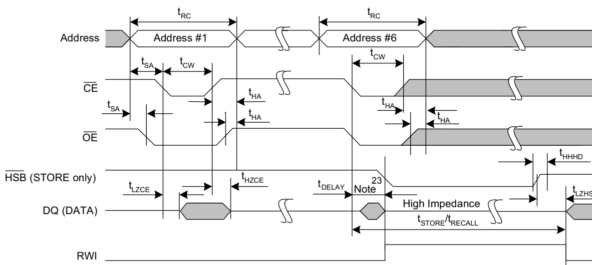
Figure 12. Autostore Enable/Disable Cycle
