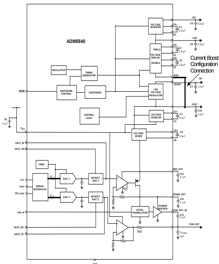
Figure 6. Current Boost Configuration
