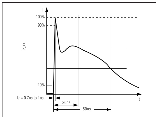
Figure 6b. IEC 1000-4-2 ESD Generator Current Waveform
