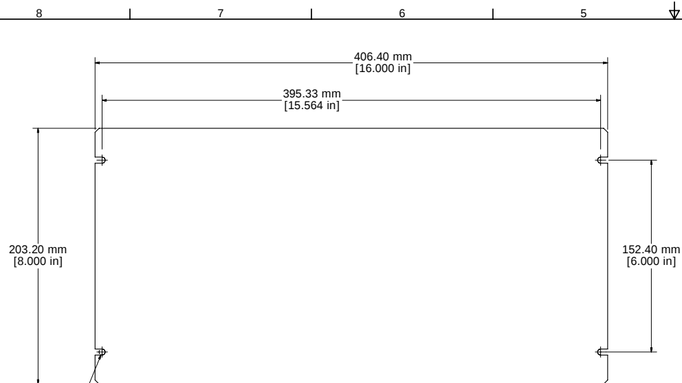
1434-26 - VIEW FROM TOP (SOLD SEPERATELY)
