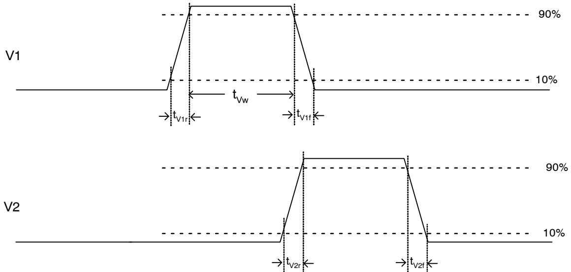
Figure 21. Frame Timing Detail
