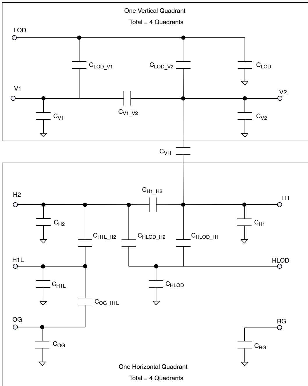
Figure 18. Capacitance Model
