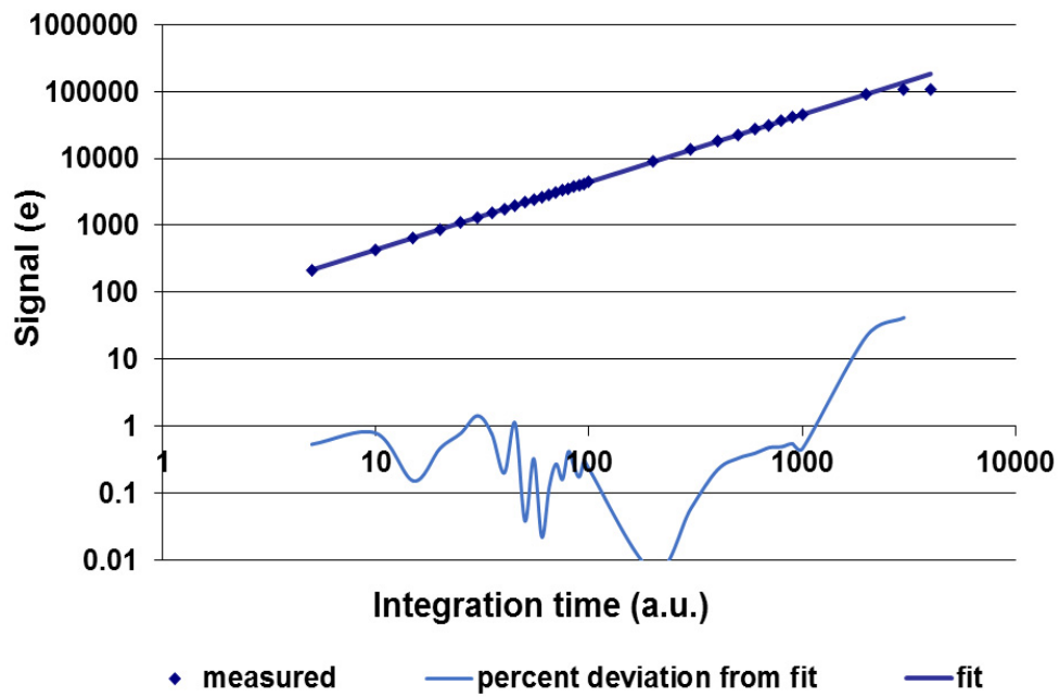
Figure 17. Typical linearity Performance: 3x3 Binned Resolution (20 MHz)
