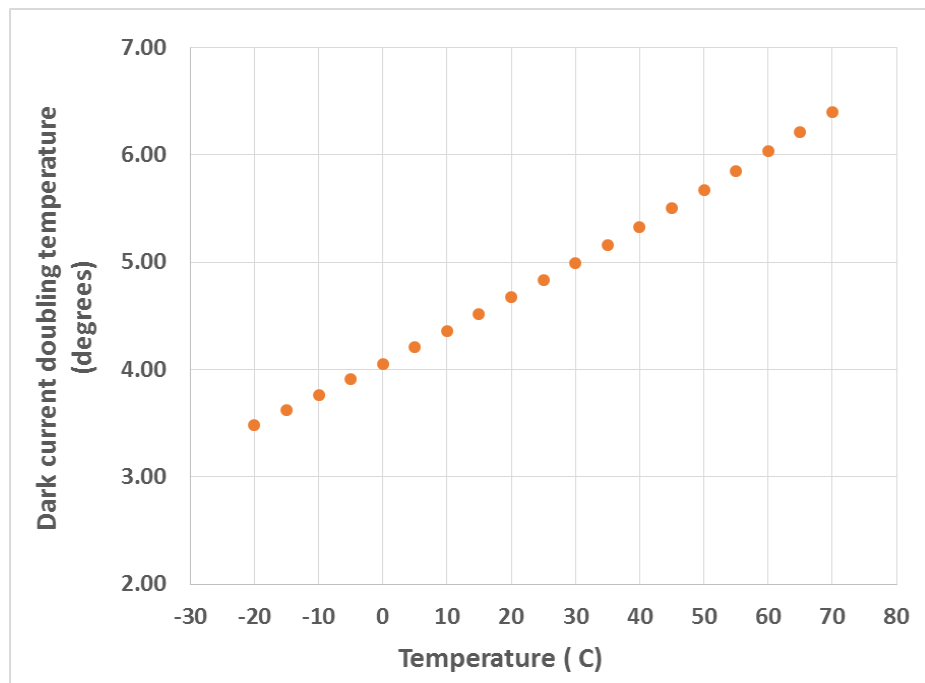
Figure 13. Dark Current Doubling Temperature
