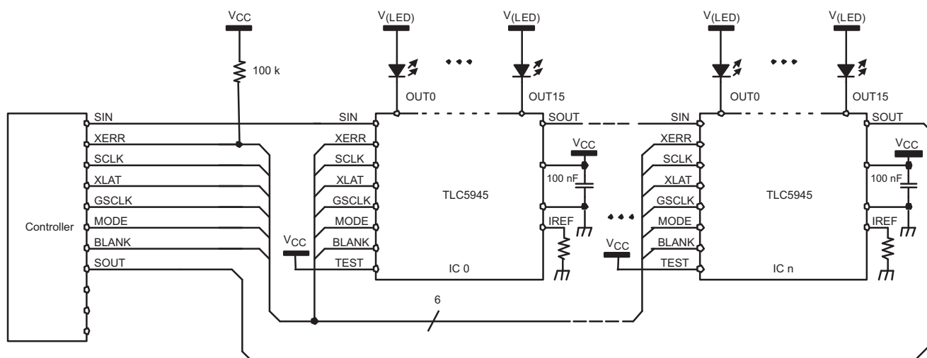
Figure 16. Cascading Devices
