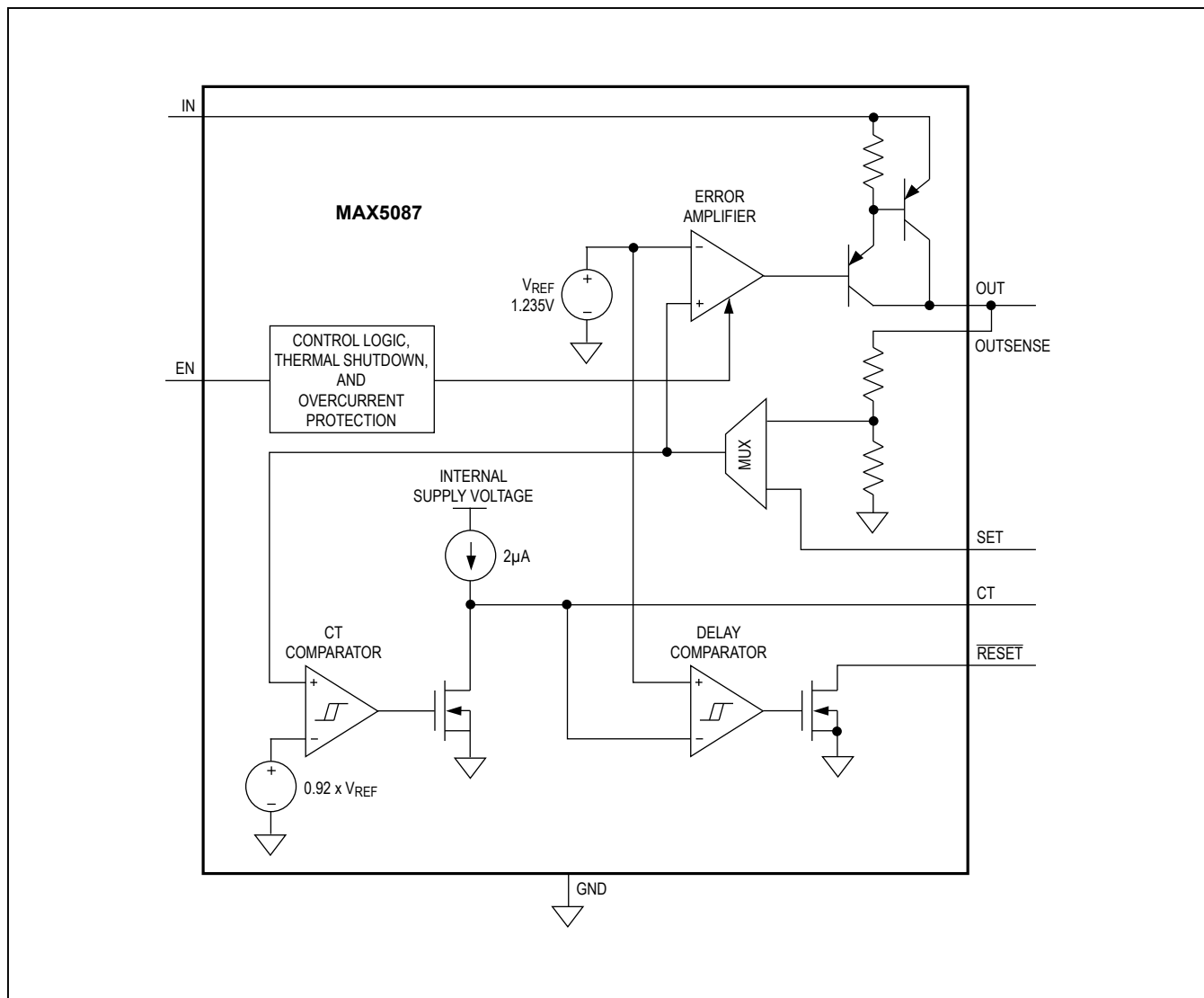
Figure 1. Functional Diagram
