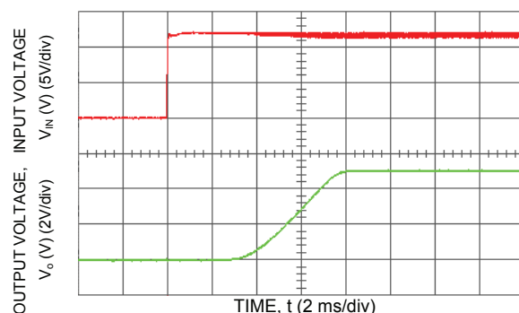
Figure 16. Typical Start-Up with application of V_{in} with low-ESR polymer capacitors at the output ( 7 \times 150\text{ }\mu\text{F} ) ( V_{in} = 12\text{ Vdc} , V_o = 5.0\text{ Vdc} , I_o = 16\text{ A} , C_o = 1050\text{ }\mu\text{F} ).
