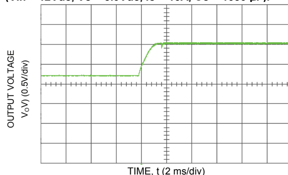
Figure 17 Typical Start-Up with Prebias ( V_{in} = 12\text{ Vdc} , V_o = 5.0\text{ Vdc} , I_o = 1\text{ A} , V_{bias} \approx 3.3\text{ Vdc} ).
