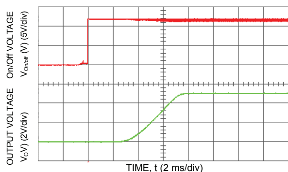
Figure 15. Typical Start-Up Using Remote On/Off with Low-ESR external capacitors ( 7 \times 150\text{ }\mu\text{F} Polymer) ( V_{in} = 12\text{ Vdc} , V_o = 5.0\text{ Vdc} , I_o = 16\text{ A} , C_o = 1050\text{ }\mu\text{F} ).
