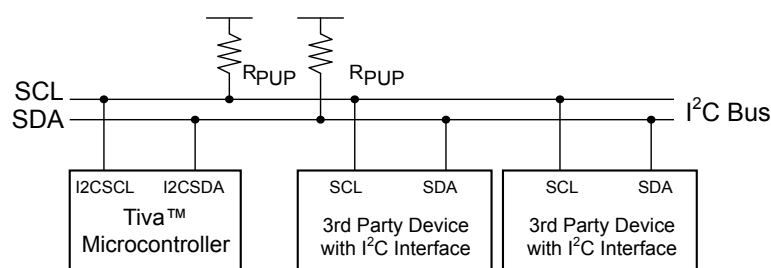
Figure 21-2. I 2 C Bus Configuration
