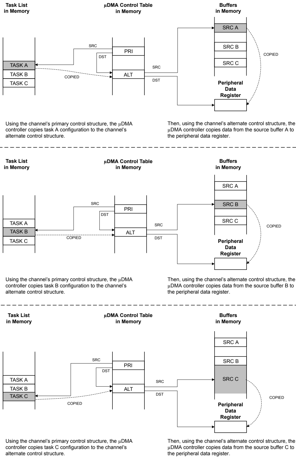
Figure 9-6. Peripheral Scatter-Gather, \mu DMA Copy Sequence
