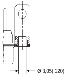
Plastic Bracket with Bushing (1A5N)
