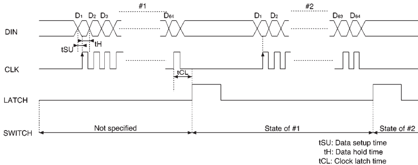
Fig. 2 Timing waveform
