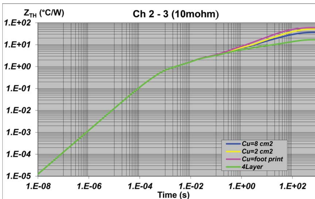
Figure 31. PowerSSO-36 thermal impedance junction ambient single pulse
