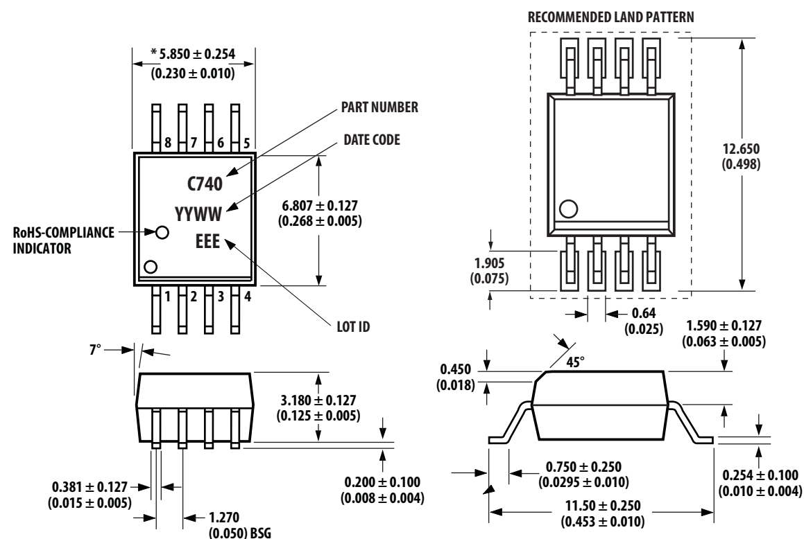
Figure 3: Package Dimensions
