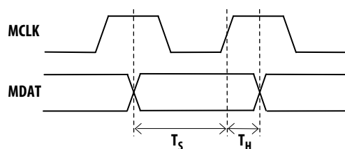
Figure 4: Data Timing
