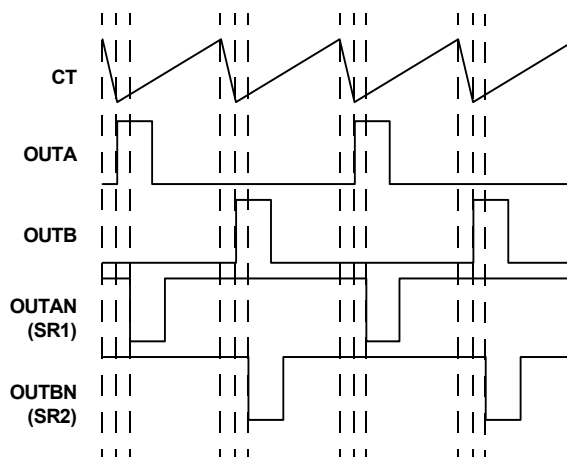
FIGURE 16. WAVEFORM TIMING WITH SR OUTPUTS DELAYED, 2.575\text{V} < \text{VADJ} < 5.00\text{V}
