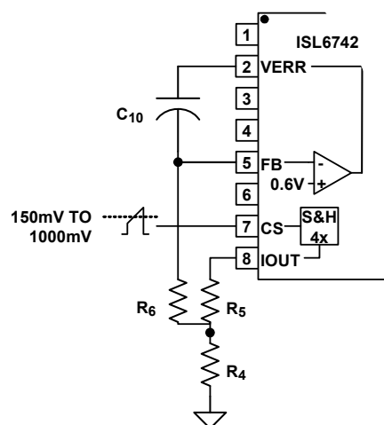
FIGURE 10. AVERAGE OVERCURRENT IMPLEMENTATION
