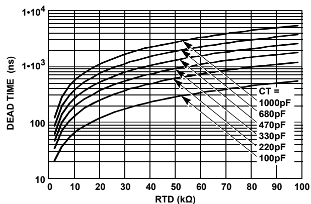
FIGURE 6. DEAD TIME (DT) vs CAPACITANCE
