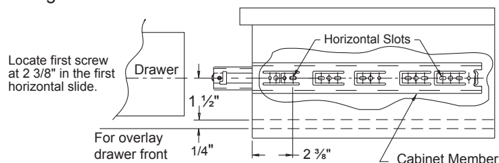
Figure 1 Conventional Mounting—Cabinet
