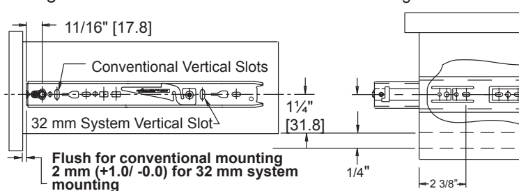
Figure 4 Conventional and 32 mm Mounting—Drawer
