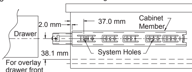
Figure 2 32 mm Mounting—Cabinet
