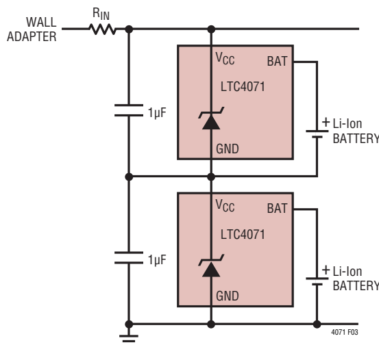
Figure 3. 2-Cell Battery Charger
