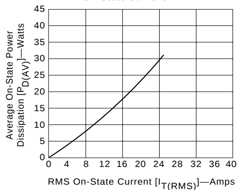
Power Dissipation (Typical) vs On-State Current
