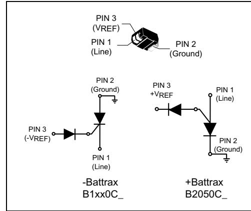
Electrical Parameters (Preliminary Data for Positive Tracking Devices)
