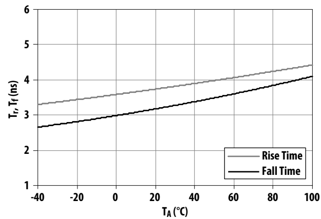
Figure 9: Typical Rise and Fall Time vs Temperature at 3.3V Supply Voltage
