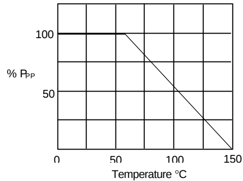
Figure 4 - Derating Curve
