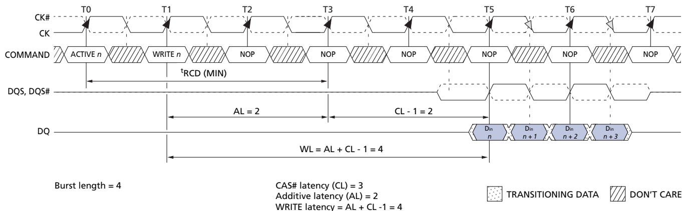
Figure 9: Write Latency
