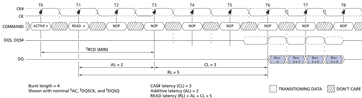
Figure 8: READ Latency
