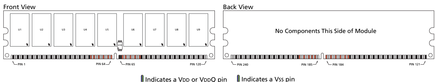
Figure 2: Pin Locations
