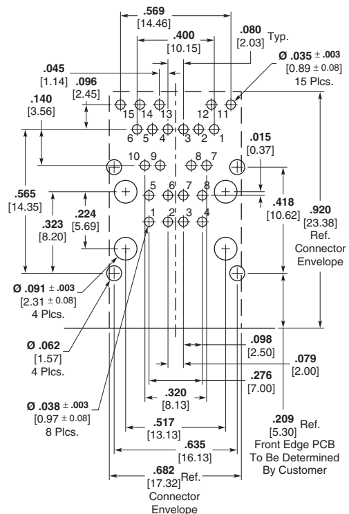
PCB Footprint
