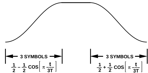
Figure 11. Ramp Envelope
