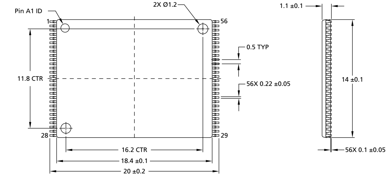
Figure 32: 56-Pin TSOP – 14mm x 20mm
