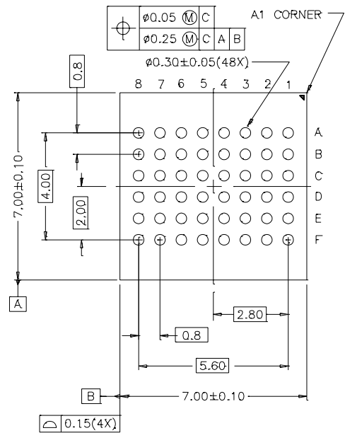
BOTTOM VIEW
