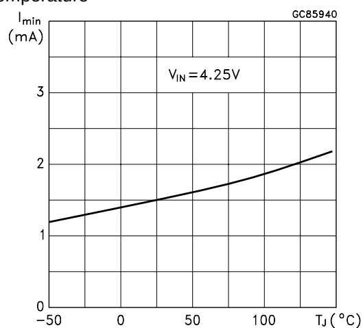
Figure 20: Minimum Load Current vs Temperature
