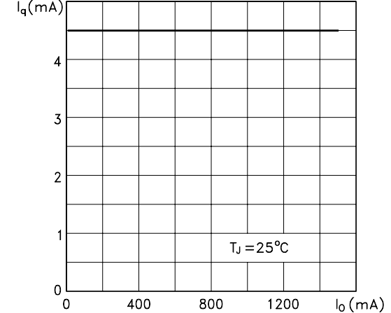
Figure 15: Quiescent Current vs Output Current
