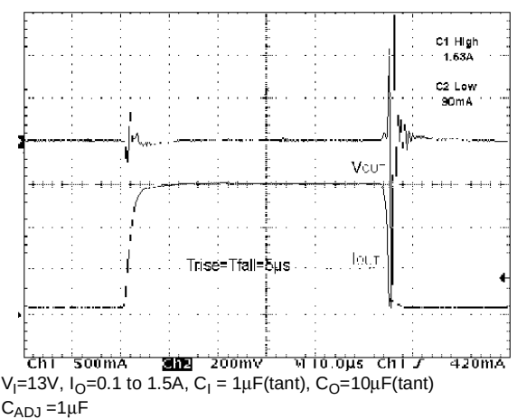
Figure 27: Load Transient
