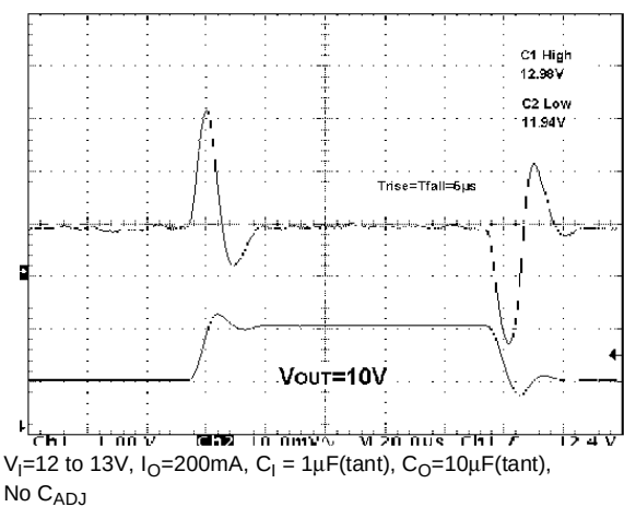
Figure 24: Line Transient
