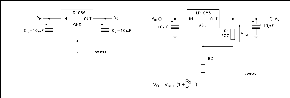
Figure 2: Application Circuits
