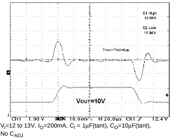
Figure 26: Line Transient
