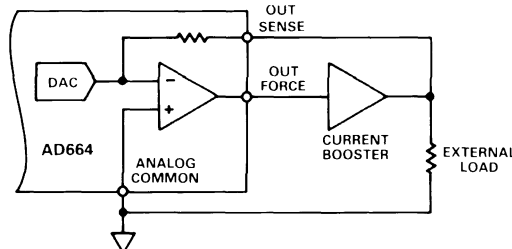
Figure 3. Current-Boosting Scheme
