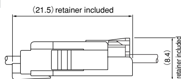
PA Receptacle (Standard type) + PAL Receptacle
