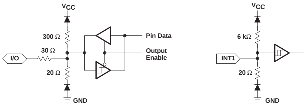
Figure 21. Typical Buffer Circuitry
