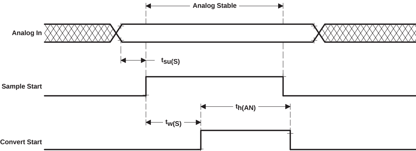
Figure 33. Analog Timing
