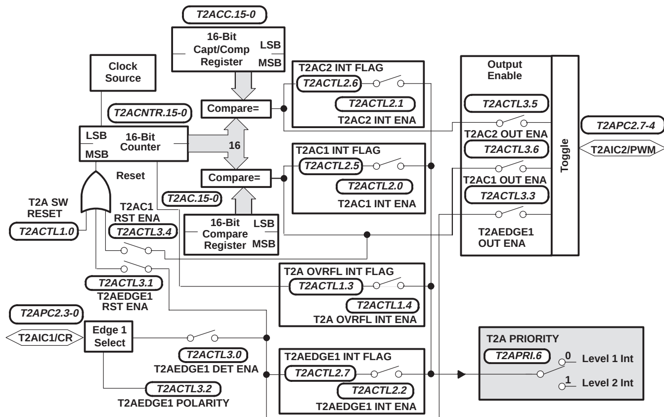
Figure 12. Dual-Compare Mode
