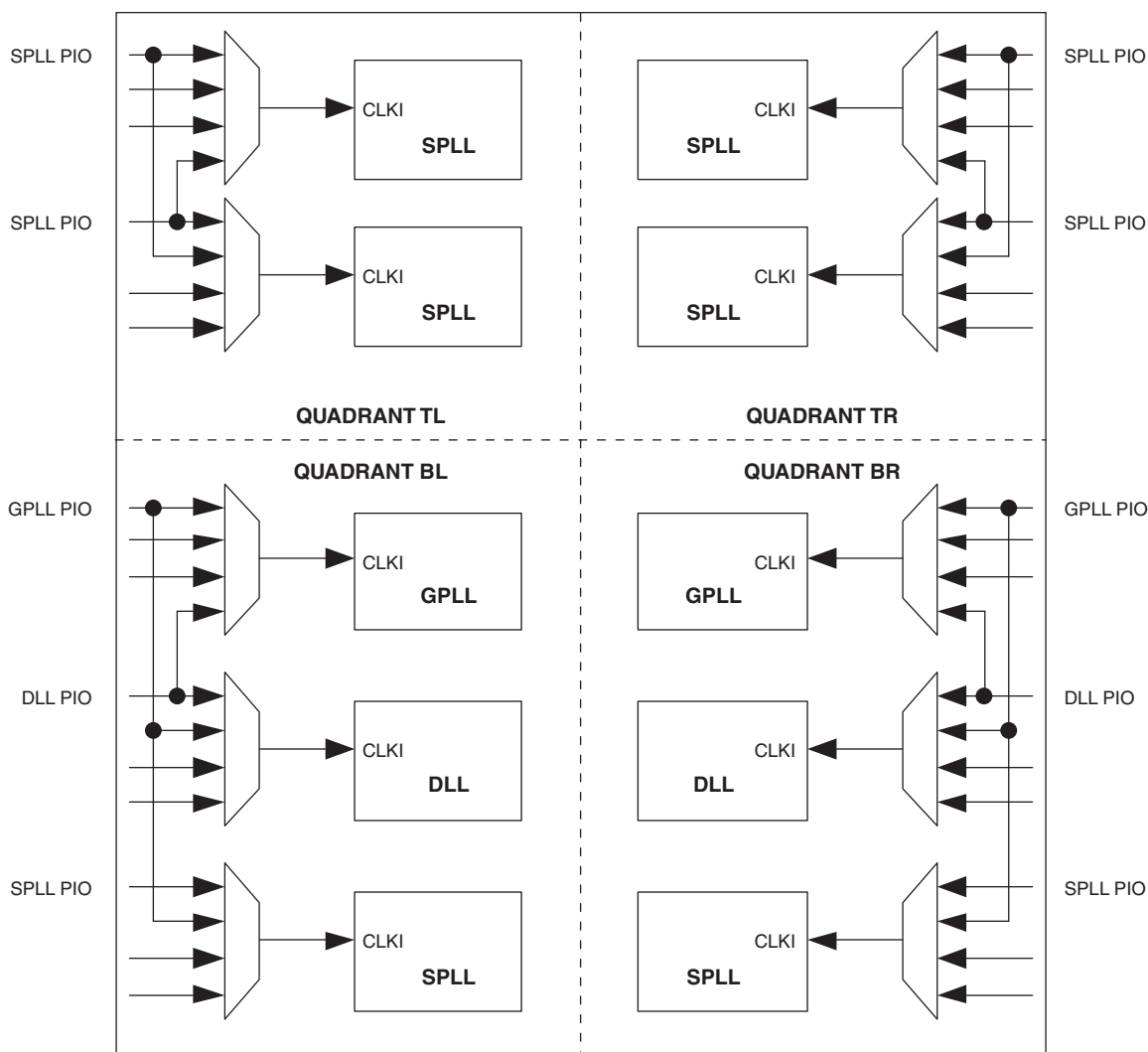
Figure 10-31. Input Clock Sharing (LatticeECP2M with Six SPLs)
