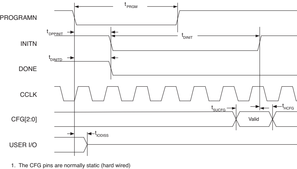
Figure 3-18. Configuration from PROGRAMN Timing
