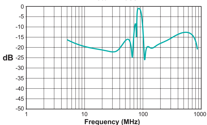
Return Loss
