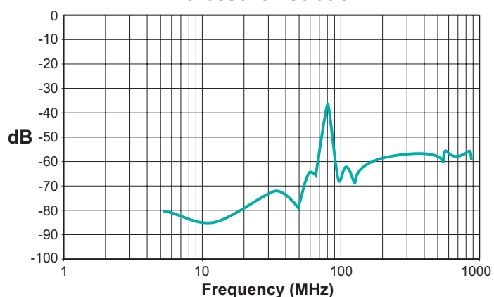
Crossover Isolation
