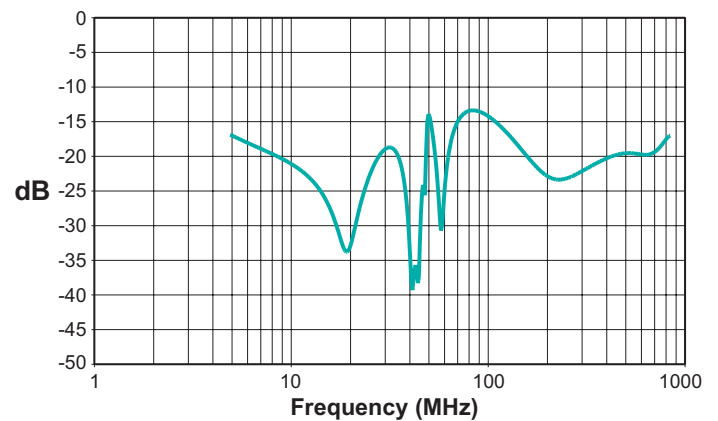
Return Loss
