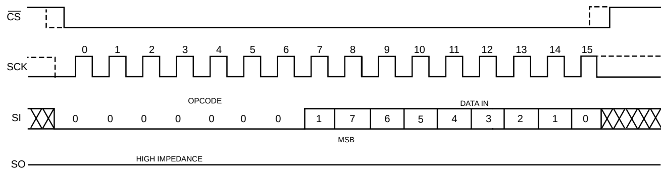
Figure 7. WRSR Timing
