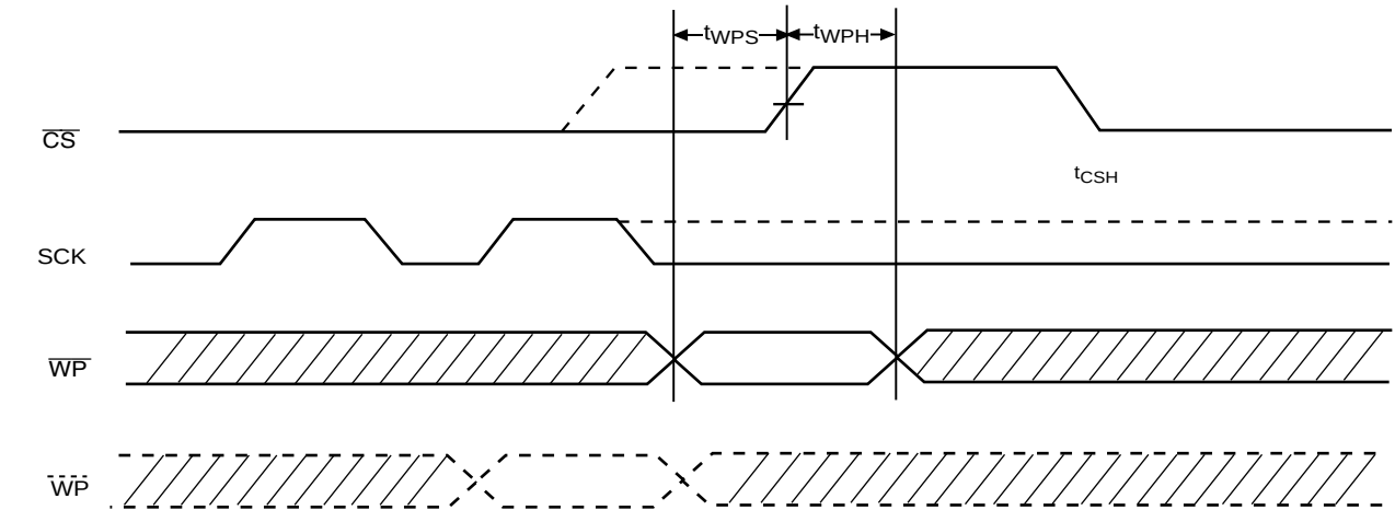
Figure 10. WP Timing
