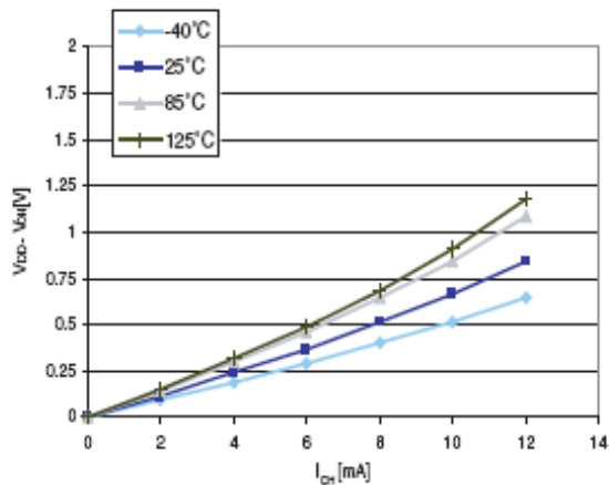
Figure 33. Typ. V_{DD} - V_{OH} @ V_{DD} = 3.3\text{ V} (high sink ports)
